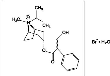
Figure 3.1-2. Chemical structure of ipratropium bromide.
